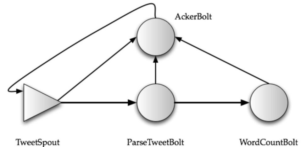
Figure 2: High Level Architecture of Storm
