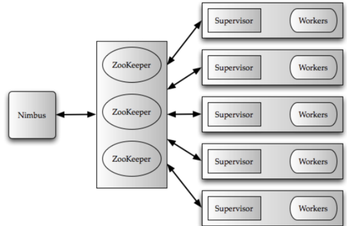
Figure 2: High Level Architecture of Storm
